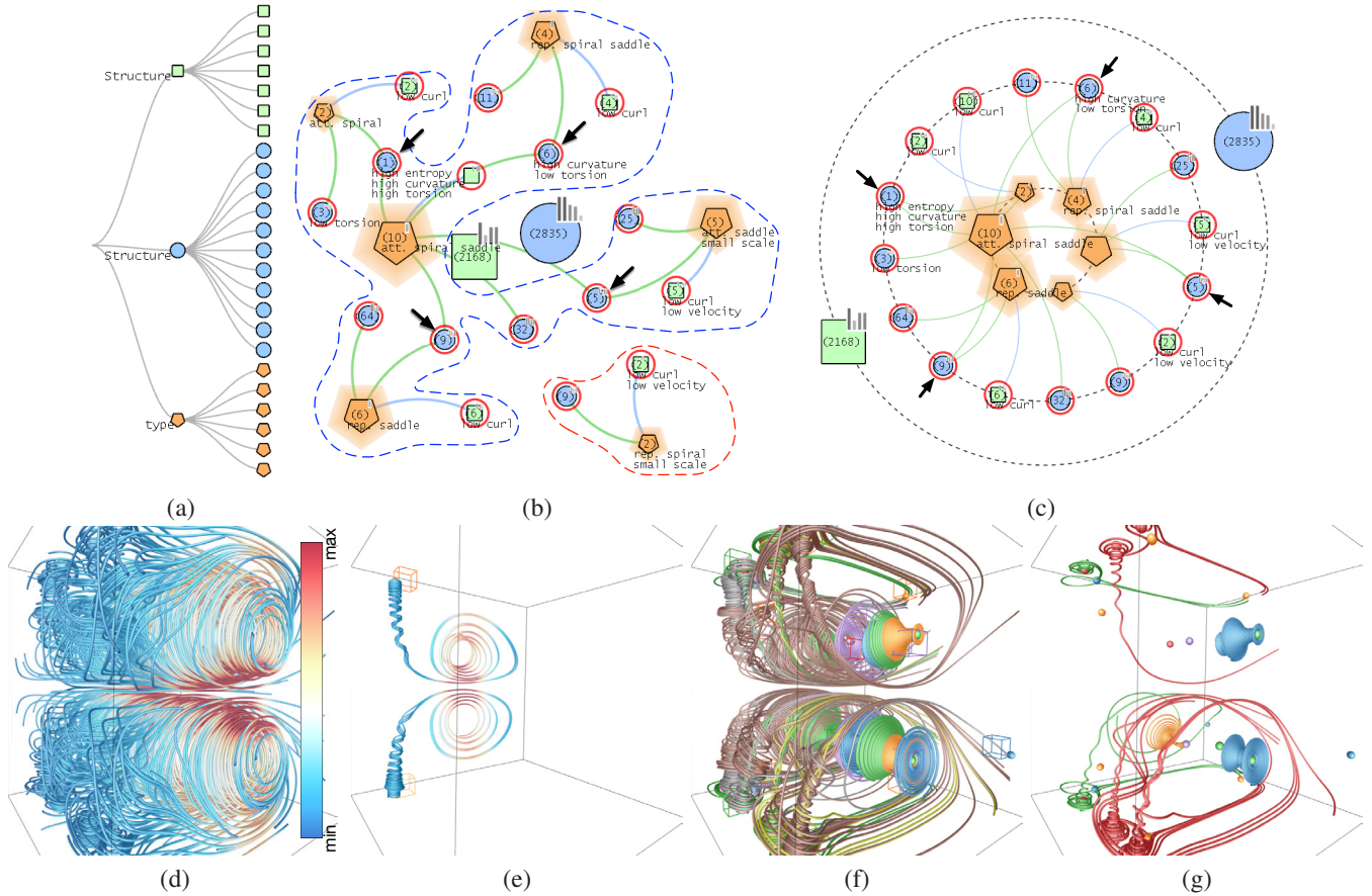
Fig. 5: Exploration of the two swirls data set. (a) The node split history. (b) Neighborhood inspection for all P-nodes without the egocentric layout. Each P-node represents a type of critical points. (c) The same inspection result of (b) with the egocentric layout. (d) 300 streamlines randomly selected from the entire pool of 3000 streamlines. The velocity magnitude is mapped to streamline colors. (e) and (f) The objects in the red and blue dashed boundaries of (b), respectively. (g) The connectors of the P-nodes.
